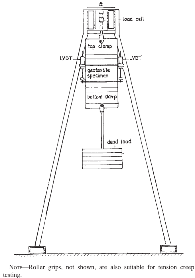
FIG. X2.2 Geotextile Loading System
