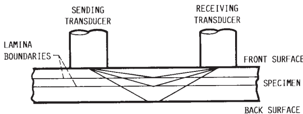
(B) FIRST ORDER LONGITUDINAL (P-WAVE) RAY PATHS IN LAMINATED SOLID.
