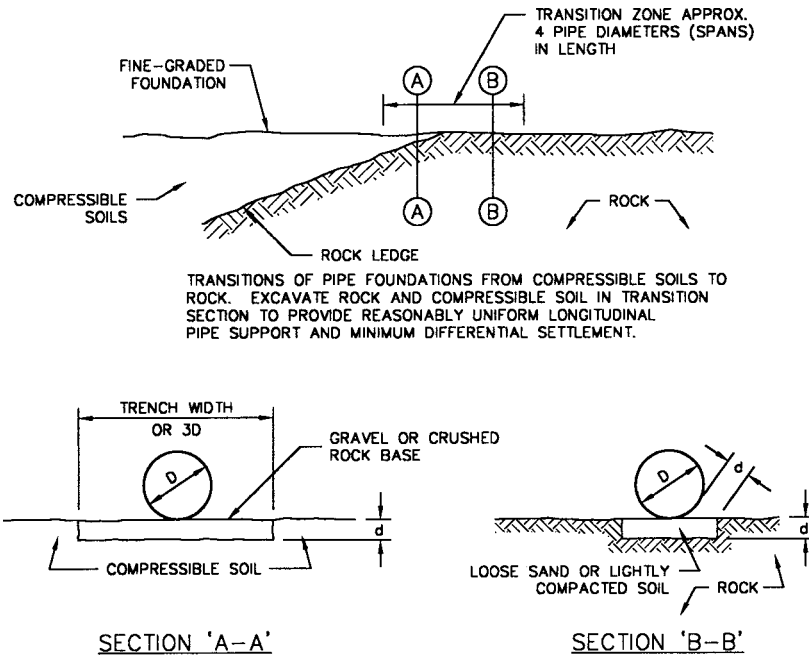
FIG. 3 Foundation Transition Zones and Rock Foundations
