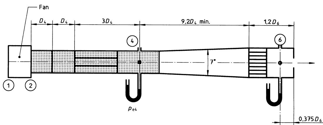
b) Flowrate determination using outlet orifice
