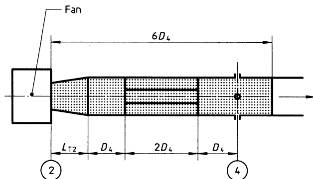
Figure 55 — Circular fan outlet for D_2 \neq D_4
