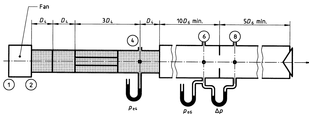
c) Flowrate determination using in-duct orifice with taps at D and 0.5D or in-duct orifice with corner taps
