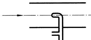
Figure 53 — Pitot-static traverse for flowrate determination (see clause 27)
