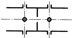
Figure 48 — In-duct orifice with taps at D and D/2 (see clause 26)
