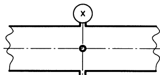
Figure 32 — Symbol for a group of wall tapplings
