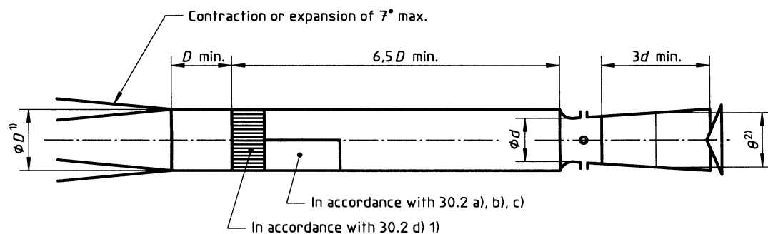
a) In-duct Venturi nozzle
