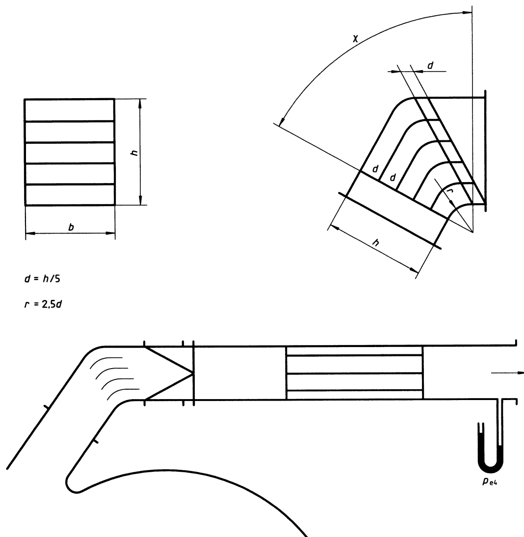
Figure D.1 — Dimensions of outlet elbow for testing large centrifugal fans
