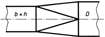
Figure 41 — Symbol for transition section joining cylindrical duct with rectangular outlet duct
