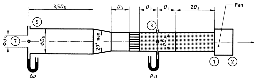
b) Flowrate determination using inlet orifice with corner taps
