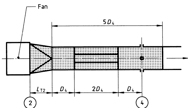
Figure 56 — Rectangular fan outlet where b > h
