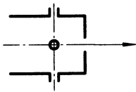
Figure 50 — Outlet orifice with wall taps (see clause 26)
