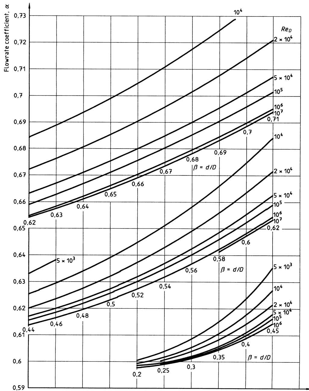
Figure 25 — Flowrate coefficient, \alpha , of in-duct or outlet orifice with corner taps (see 26.8)
