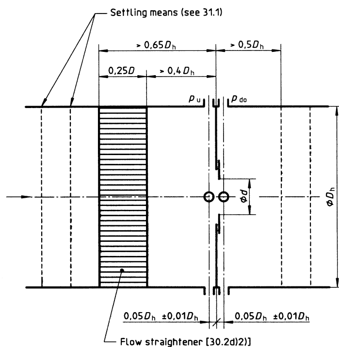
i) Orifice plate in test chamber (inlet-side or outlet-side), see 26.9.1, 31.4 and 31.3
