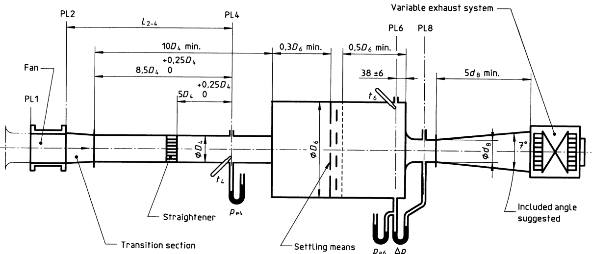
g) Flowrate determination using nozzle on end of chamber
