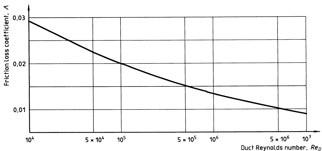
b) Friction loss coefficient for ducts (30.6.2 and 30.6.5)
