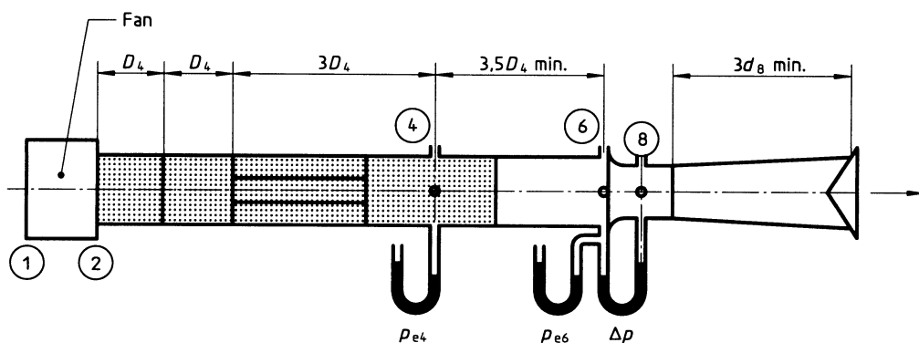
a) Flowrate determination using ISO Venturi nozzle
