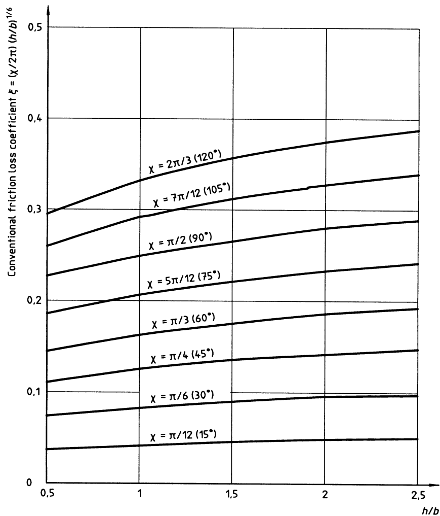
Figure D.2 — Variation \frac{\chi}{2\pi} \left(\frac{h}{b}\right)^{\frac{1}{6}} for calculating the pressure loss in an outlet elbow
