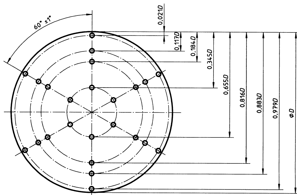
Figure 30 — Positions for traverse measurements in standardized airways
