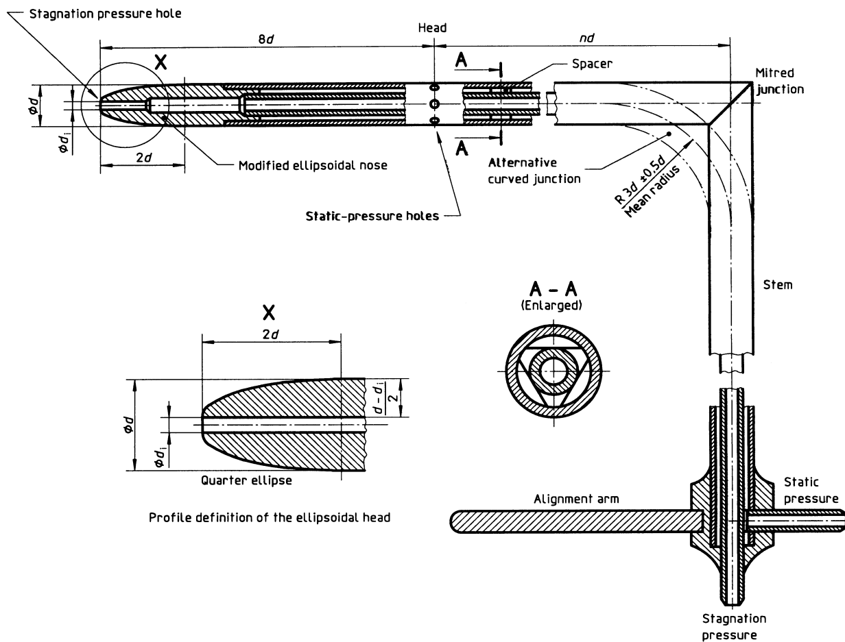
b) NPL type with modified ellipsoidal nose
