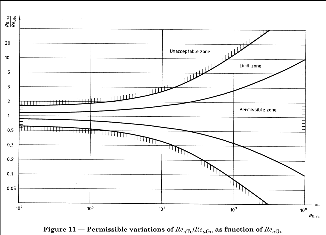
Figure 11 — Permissible variations of Re_{uTe}/Re_{uGu} as function of Re_{uGu}
