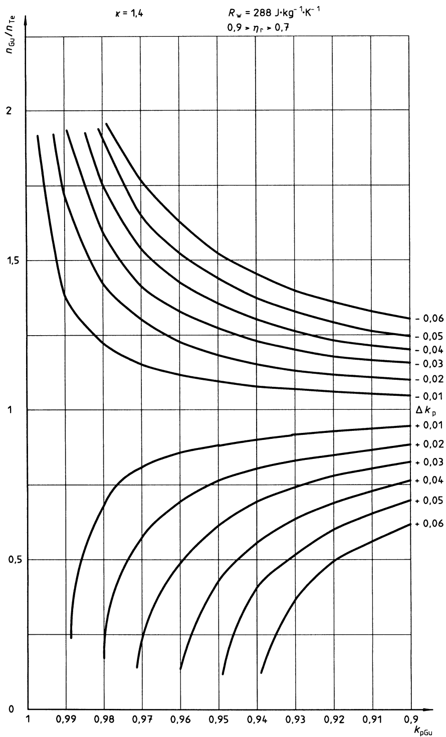
Figure 12 — Variation of n_{Gu}/n_{Te} as a function of k_{pGu} and \Delta k_p
