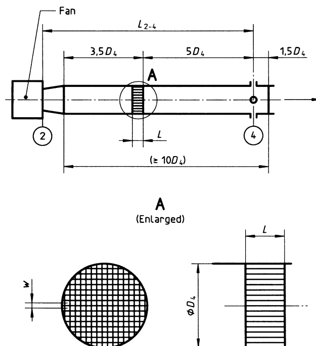
Figure 57 — Circular or rectangular fan outlet where 0,95 \leq A_2/A_4 \leq 1,05
