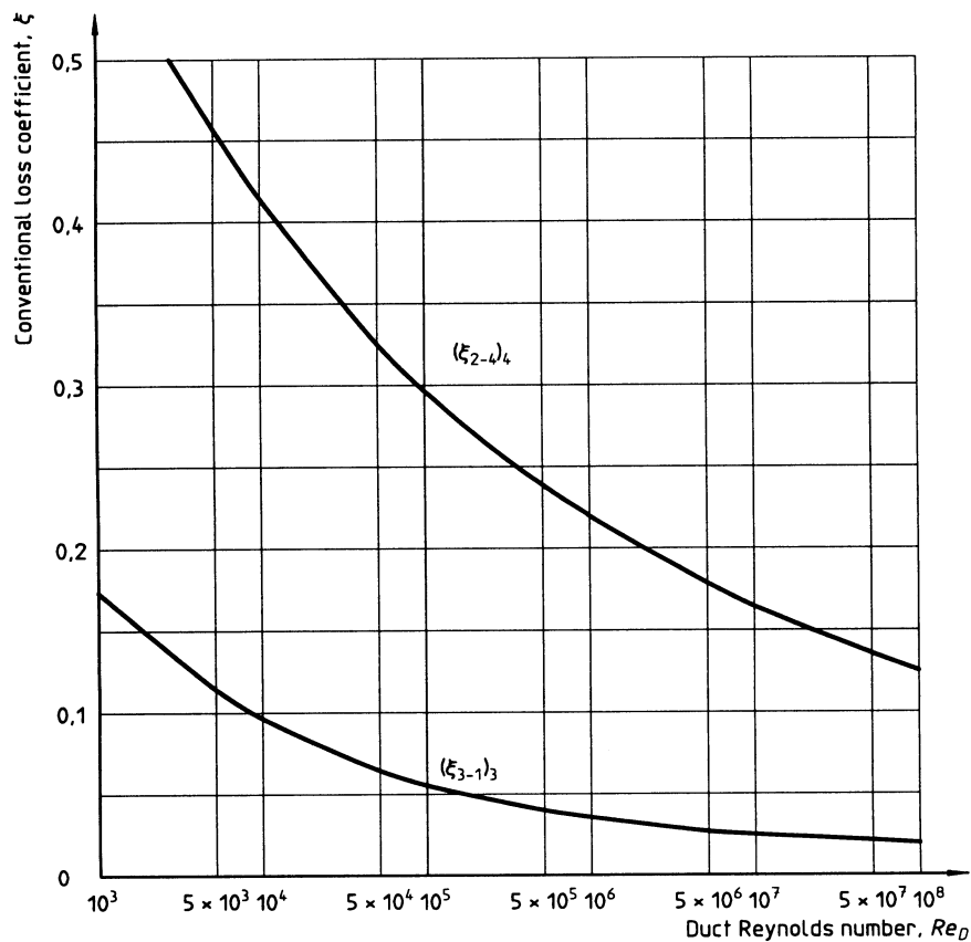
a) Conventional loss coefficient for standardized airways (30.6.1 and 30.6.4)
