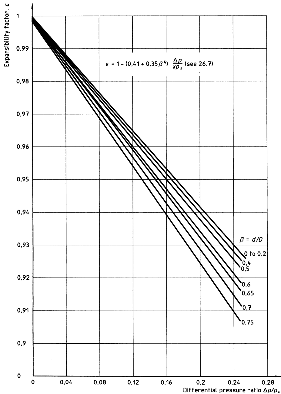
Figure 26 — Expansibility factor, \epsilon , for orifice plates in atmospheric air (see 26.7, 26.8 and 26.10)
