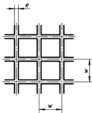
j) Detail of flow straightener
