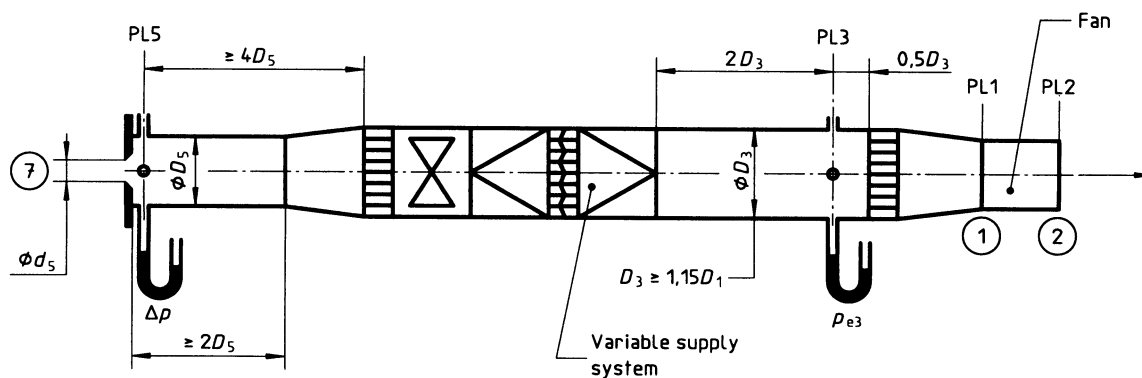
c) Flowrate determination using inlet orifice with wall tapings
