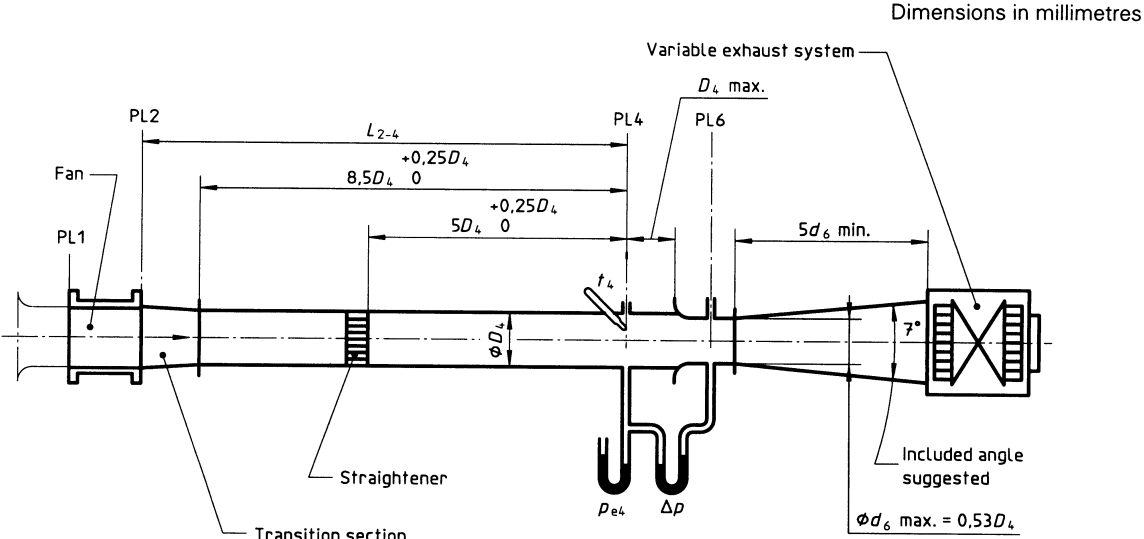
f) Flowrate determination using in-duct Venturi nozzle
