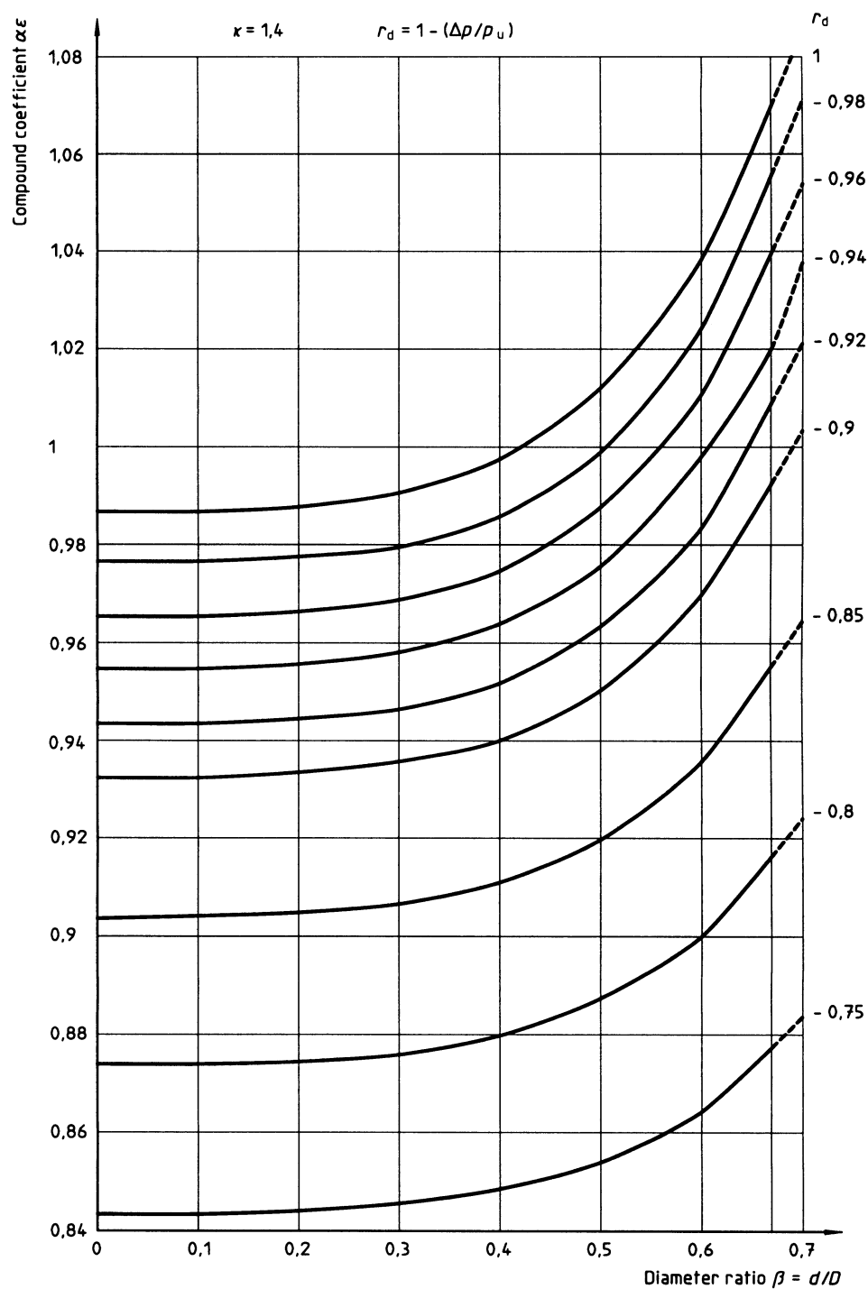
Figure 18 — Compound flow coefficients of ISO Venturi nozzles
