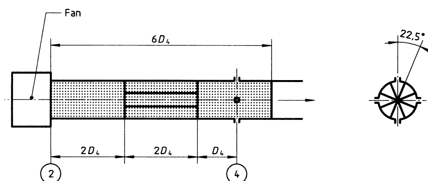
Figure 54 — Circular fan outlet for D_2 = D_4
