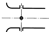
Figure 46 — Quadrant inlet nozzle (see clause 24)
