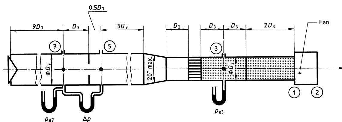
e) Flowrate determination using in-duct orifice with taps at D and 0.5D or in-duct orifice with corner taps
