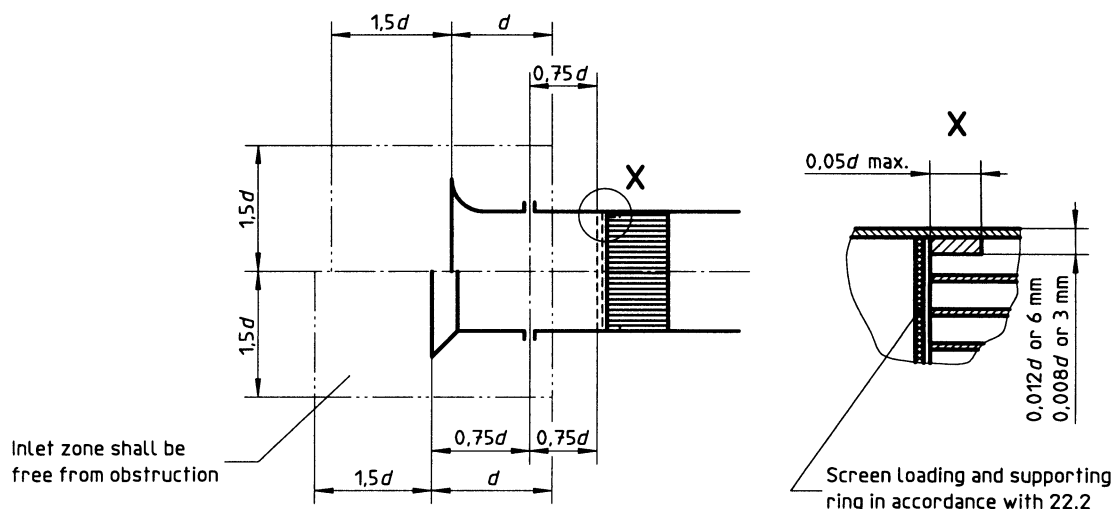
c) Free-inlet Venturi nozzle or conical inlet with adjustable screen loading
