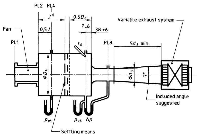
a) Flowrate determination using Ventutrl nozzle on end of chamber
