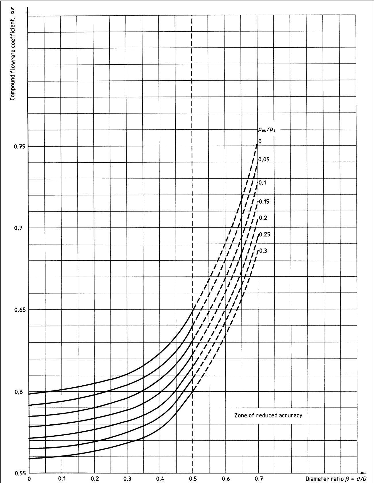
Figure 27 — Compound flowrate coefficient, \alpha\epsilon , of outlet orifices with wall taps (see 26.9)
