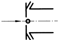
Figure 51 — Inlet orifice with corner taps (see clause 26)
