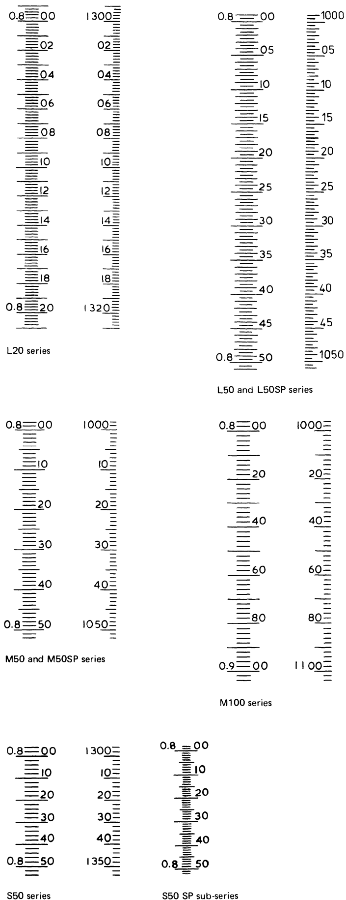
Figure 2 — Examples of hydrometer scales recommended in clause 10
